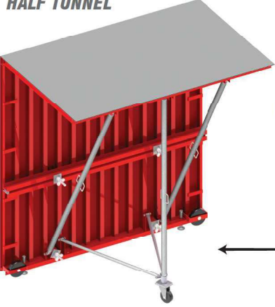
YARIM TÜNEL HALF TUNNEL
